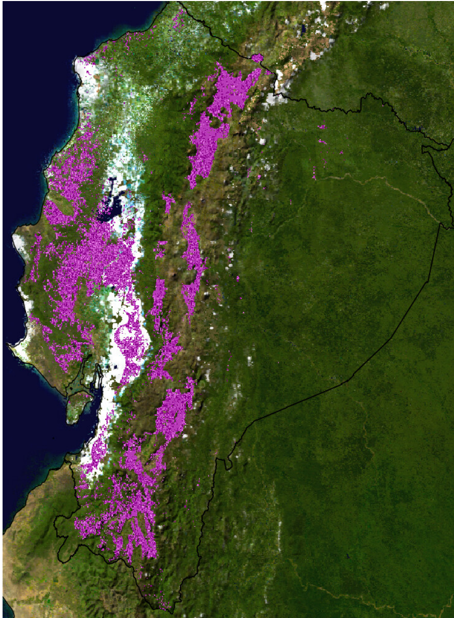
Figure 2: Area deemed available for forest restoration. Areas in purple indicate the 1 km 2 planning units that were assessed to have potential for forest restoration given (see Methods for details). The shading of cells from light to dark purple is proportional to the area within each planning unit available for forest restoration.
