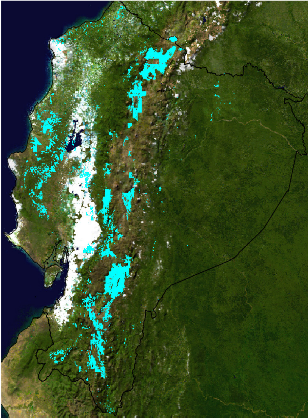
Figure 17: Restoration of 50% of deforested lands. Priority locations for restoration (cyan) for a solution that represents a balance between climate change mitigation and biodiversity conservation objectives while maximising cost-effectiveness (benefit/cost).
