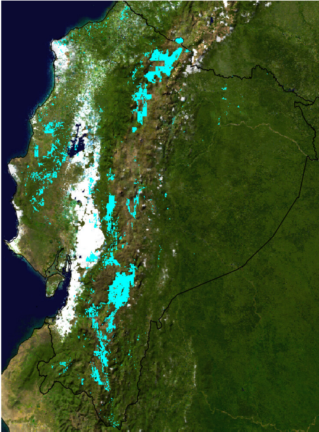
Figure 14: Restoration of 40% of deforested lands. Priority locations for restoration (cyan) for a solution that represents a balance between climate change mitigation and biodiversity conservation objectives while maximising cost-effectiveness (benefit/cost).
