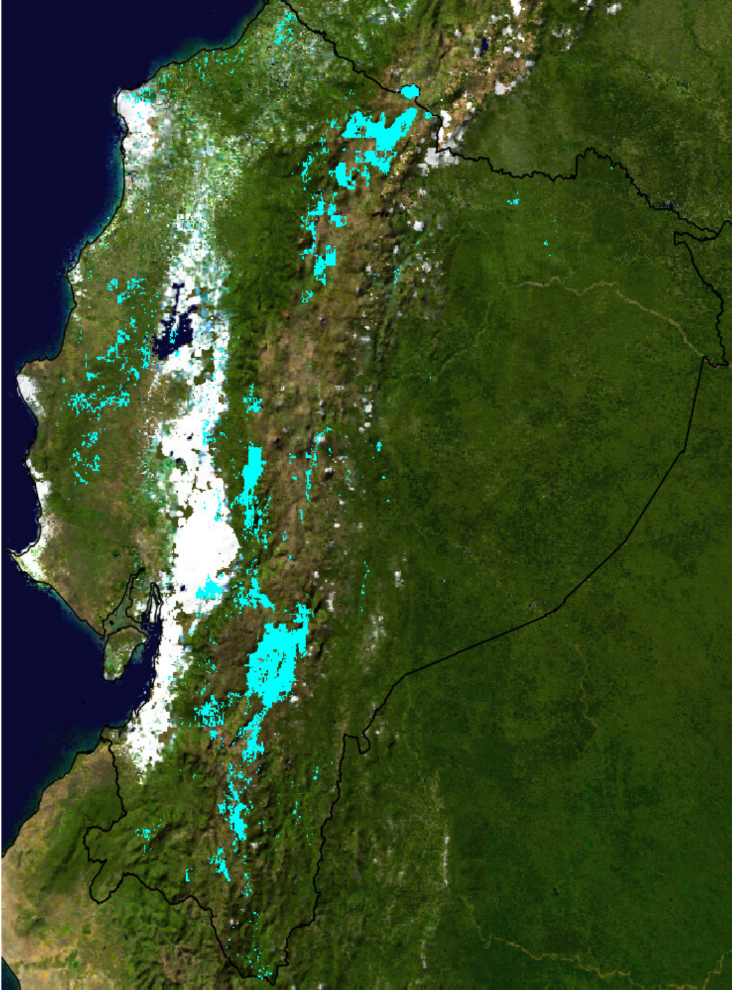
Figure 11: Restoration of 30% of deforested lands. Priority locations for restoration (cyan) for a solution that represents a balance between climate change mitigation and biodiversity conservation objectives while maximising cost-effectiveness (benefit/cost).
