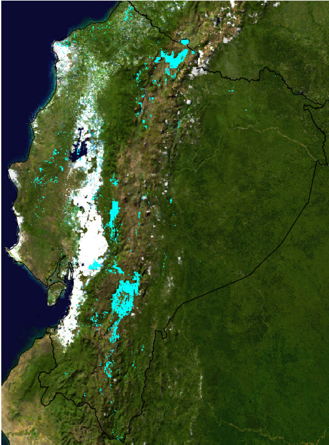
Figure 8: Restoration of 20% of deforested lands. Priority locations for restoration (cyan) for a solution that represents a balance between climate change mitigation and biodiversity conservation objectives while maximising cost-effectiveness (benefit/cost).
