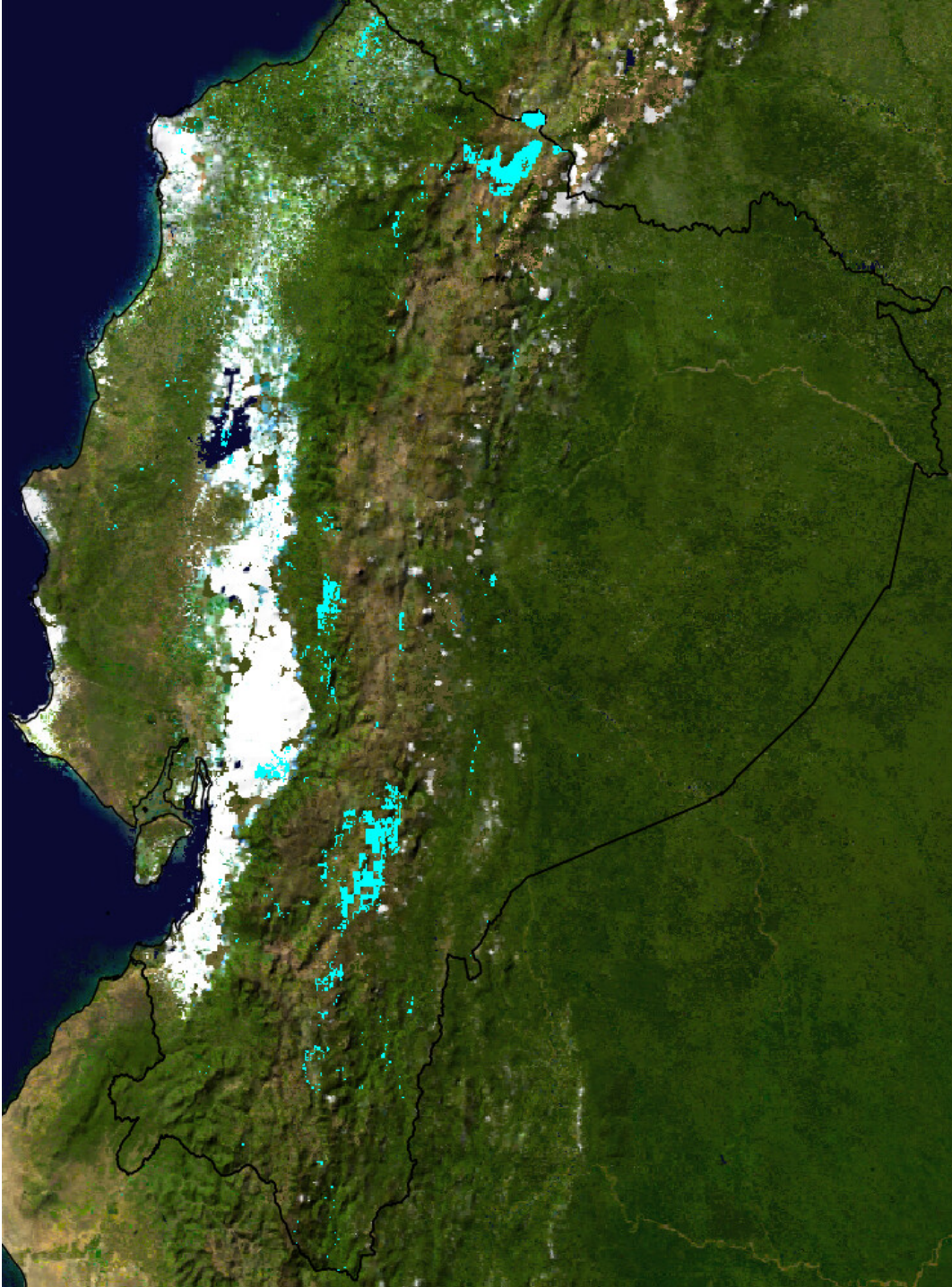
Figure 5: Restoration of 10% of deforested lands. Priority locations for restoration (cyan) for a solution that represents a balance between climate change mitigation and biodiversity conservation objectives while maximising cost-effectiveness (benefit/cost).
