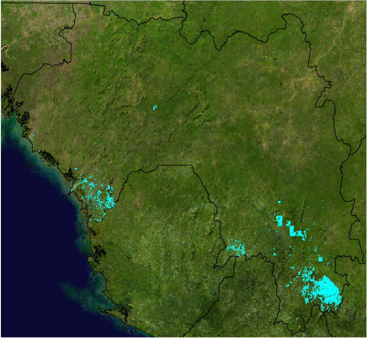
Figure 5: Restoration of 10% of deforested lands. Priority locations for restoration (cyan) for a solution that represents a balance between climate change mitigation and biodiversity conservation objectives while maximising cost-effectiveness (benefit/cost).
