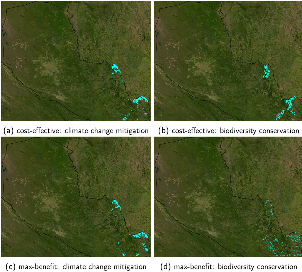
Figure 6: Restoration of 10% of deforested lands. Priority locations for restoration (cyan), under four scenarios: maximising cost-effectiveness for climate change mitigation only (a) and biodiversity conservation only (b), versus maximising benefit irrespective of cost for climate change mitigation only (c) and biodiversity conservation only (d). These figures illustrate how priority location change across the four scenarios.
