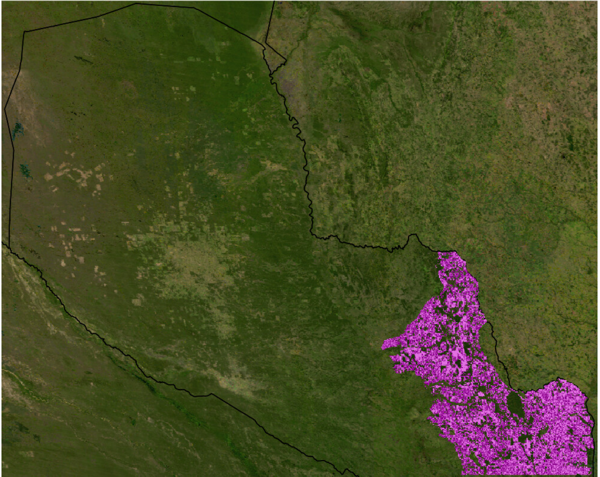
Figure 2: Area deemed available for forest restoration. Areas in purple indicate the 1 km 2 planning units that were assessed to have potential for forest restoration given (see Methods for details). The shading of cells from light to dark purple is proportional to the area within each planning unit available for forest restoration.
