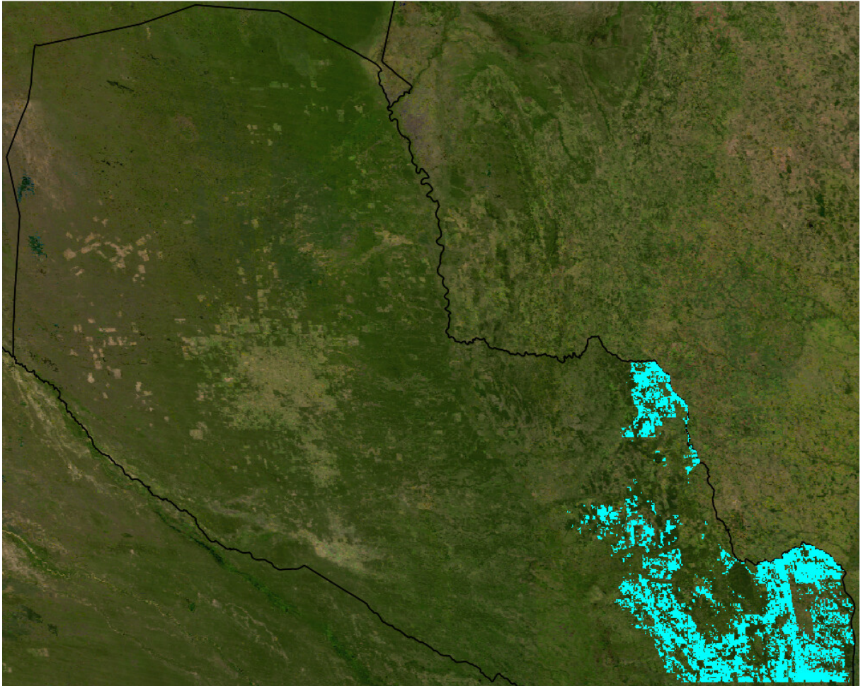
Figure 17: Restoration of 50% of deforested lands. Priority locations for restoration (cyan) for a solution that represents a balance between climate change mitigation and biodiversity conservation objectives while maximising cost-effectiveness (benefit/cost).
