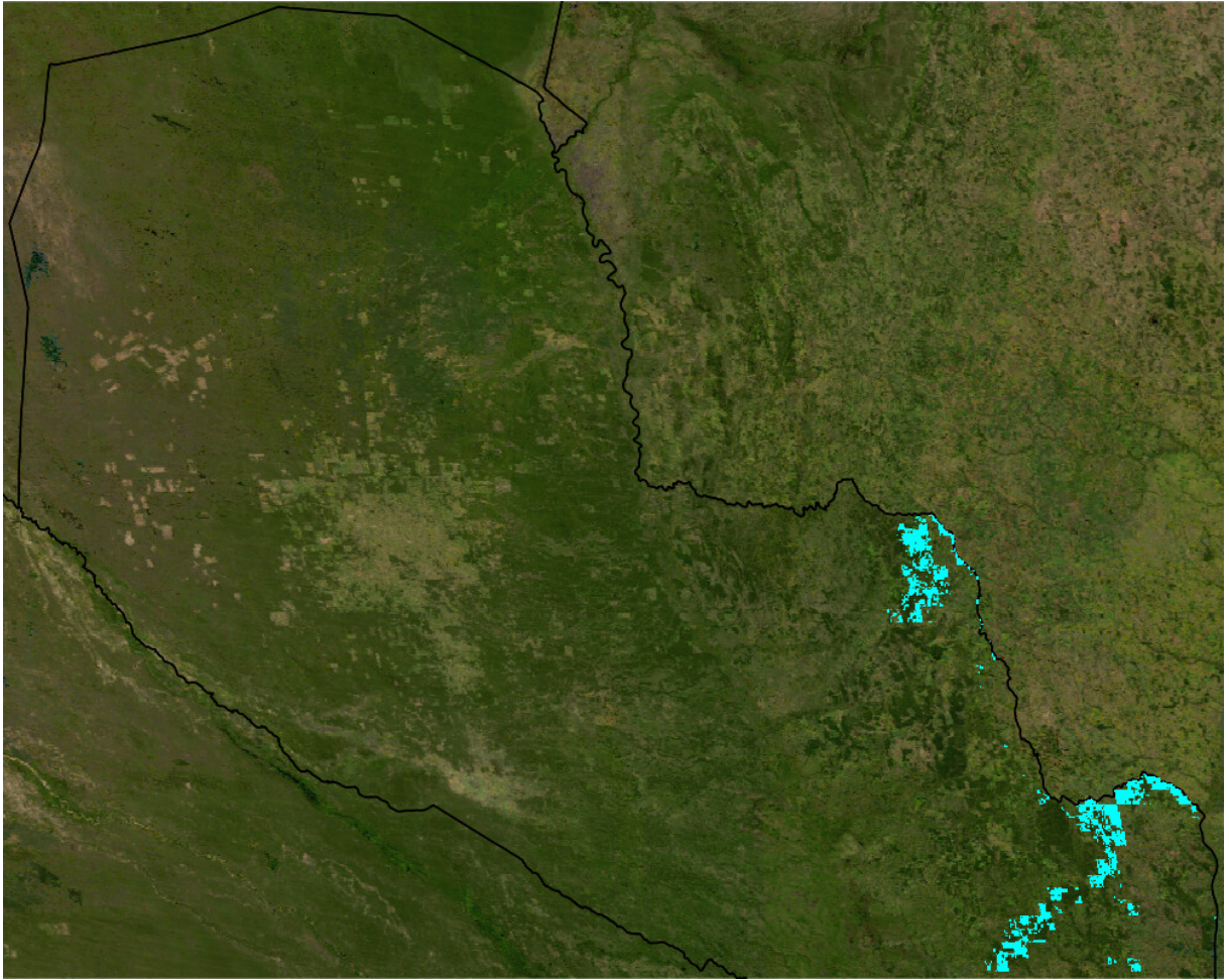
Figure 5: Restoration of 10% of deforested lands. Priority locations for restoration (cyan) for a solution that represents a balance between climate change mitigation and biodiversity conservation objectives while maximising cost-effectiveness (benefit/cost).
