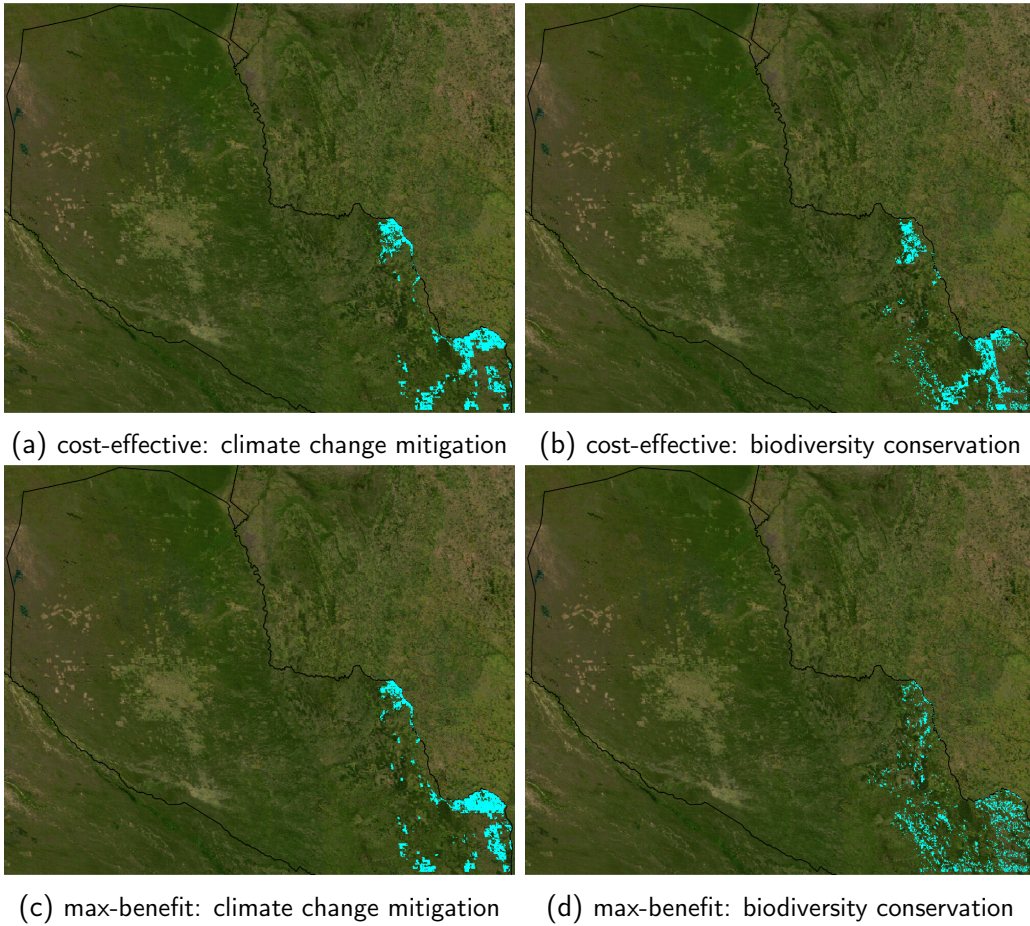
Figure 9: Restoration of 20% of deforested lands. Priority locations for restoration (cyan), under four scenarios: maximising cost-effectiveness for climate change mitigation only (a) and biodiversity conservation only (b), versus maximising benefit irrespective of cost for climate change mitigation only (c) and biodiversity conservation only (d). These figures illustrate how priority location change across the four scenarios.
