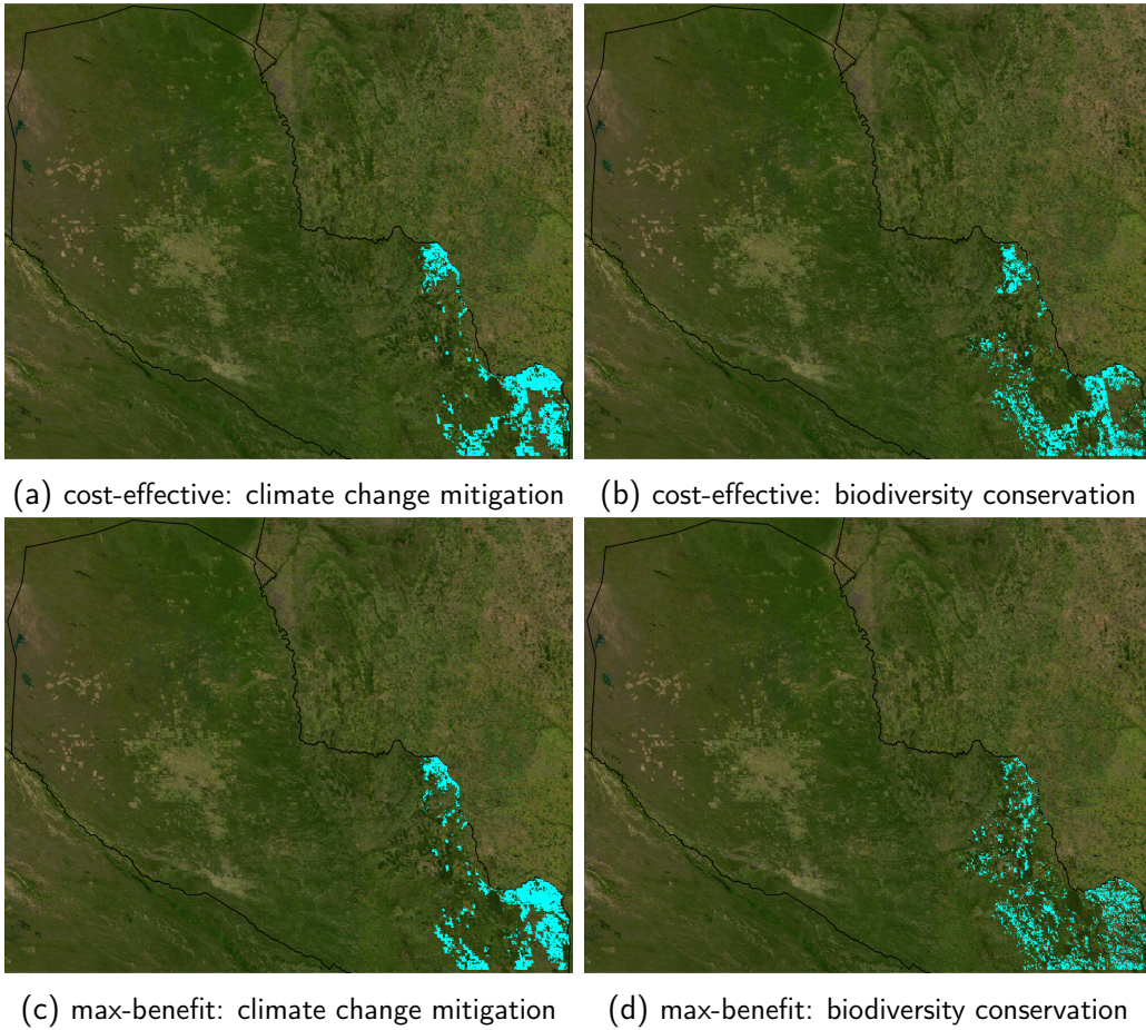
Figure 12: Restoration of 30% of deforested lands. Priority locations for restoration (cyan), under four scenarios: maximising cost-effectiveness for climate change mitigation only (a) and biodiversity conservation only (b), versus maximising benefit irrespective of cost for climate change mitigation only (c) and biodiversity conservation only (d). These figures illustrate how priority location change across the four scenarios.
