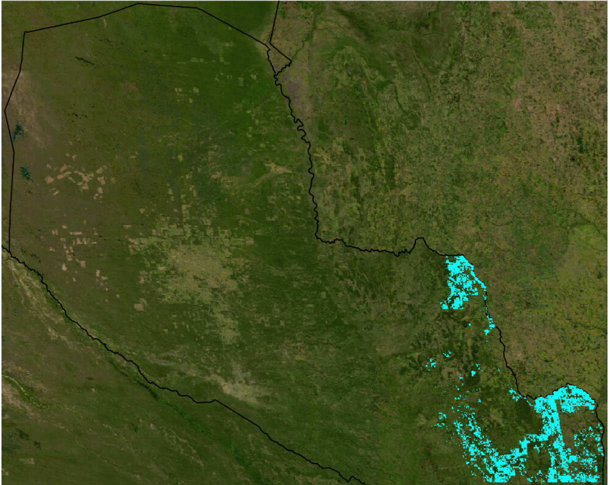
Figure 11: Restoration of 30% of deforested lands. Priority locations for restoration (cyan) for a solution that represents a balance between climate change mitigation and biodiversity conservation objectives while maximising cost-effectiveness (benefit/cost).
