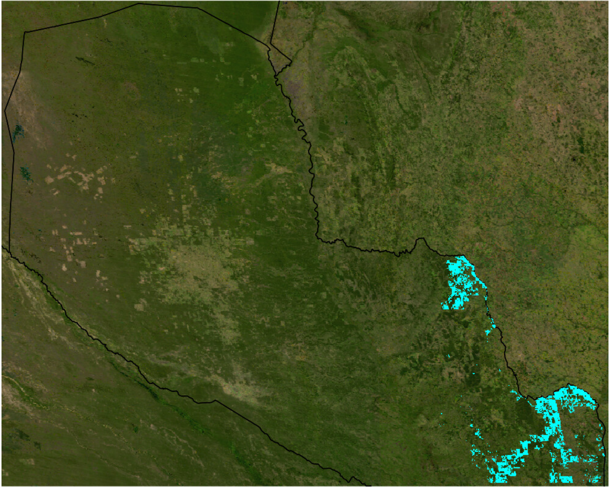
Figure 8: Restoration of 20% of deforested lands. Priority locations for restoration (cyan) for a solution that represents a balance between climate change mitigation and biodiversity conservation objectives while maximising cost-effectiveness (benefit/cost).
