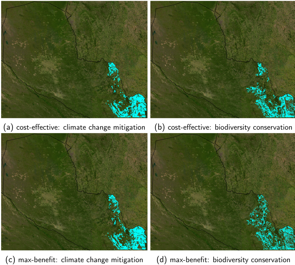
Figure 18: Restoration of 50% of deforested lands. Priority locations for restoration (cyan), under four scenarios: maximising cost-effectiveness for climate change mitigation only (a) and biodiversity conservation only (b), versus maximising benefit irrespective of cost for climate change mitigation only (c) and biodiversity conservation only (d). These figures illustrate how priority location change across the four scenarios.
