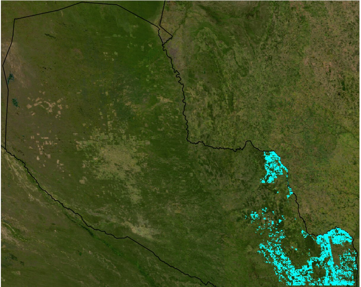
Figure 14: Restoration of 40% of deforested lands. Priority locations for restoration (cyan) for a solution that represents a balance between climate change mitigation and biodiversity conservation objectives while maximising cost-effectiveness (benefit/cost).
