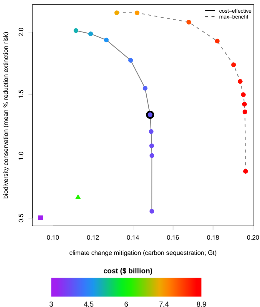
Figure 4: Restoration of 10% of deforested lands. Performance of a range of forest restoration prioritisation scenarios (points) with respect to climate change mitigation benefit (x axis), measured as above-ground carbon sequestration, and biodiversity conservation benefit (y axis), measured as the mean percent reduction in extinction risk among all species. Cost-effective scenarios (solid line) maximise return-on-investment (benefit/cost) and are likely to represent the most feasible restoration planning options. For reference, maximum-benefit scenarios (dashed line) that maximise returns irrespective of cost are also presented. The point circled in black represents a potential good compromise solution. Two further reference scenarios are also presented in which restoration is allocated randomly (triangle) or to minimise costs irrespective of benefit (square). For all scenarios the colour represents the total cost of the solution (USD; see legend). Maps of the locations associated with several of these solutions are included in the following two figures.
