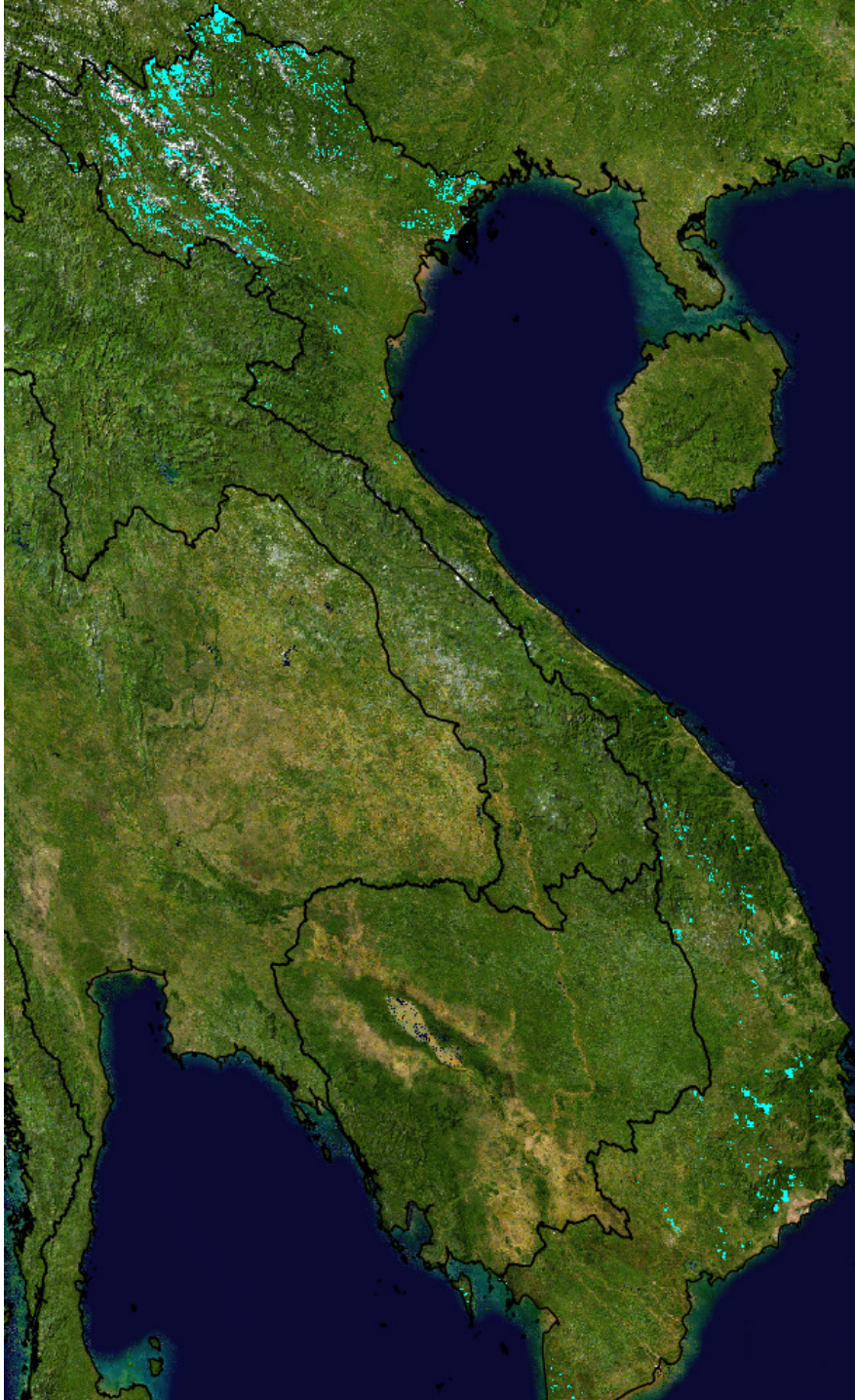
Figure 5: Restoration of 10% of deforested lands. Priority locations for restoration (cyan) for a solution that represents a balance between climate change mitigation and biodiversity conservation objectives while maximising cost-effectiveness (benefit/cost).
