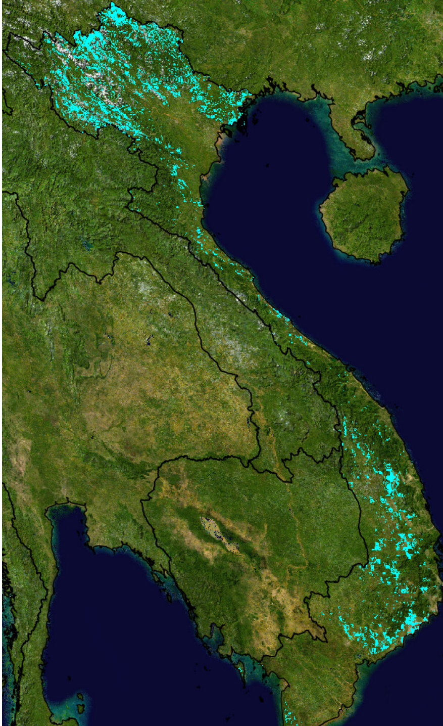
Figure 14: Restoration of 40% of deforested lands. Priority locations for restoration (cyan) for a solution that represents a balance between climate change mitigation and biodiversity conservation objectives while maximising cost-effectiveness (benefit/cost).
