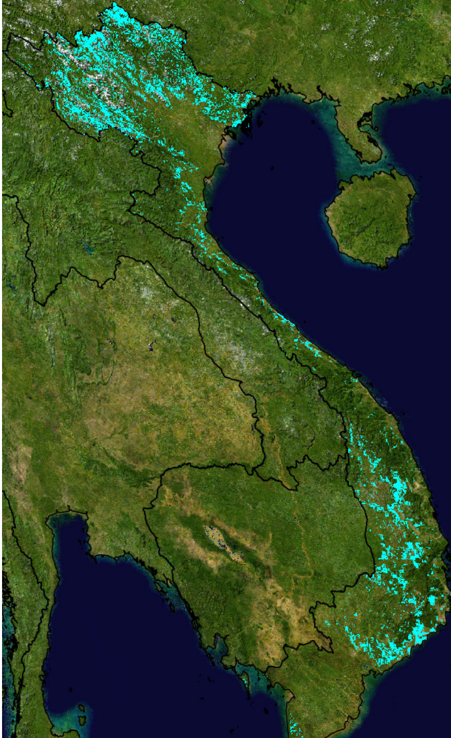
Figure 17: Restoration of 50% of deforested lands. Priority locations for restoration (cyan) for a solution that represents a balance between climate change mitigation and biodiversity conservation objectives while maximising cost-effectiveness (benefit/cost).
