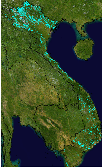
(a) cost-effective: climate change mitigation
