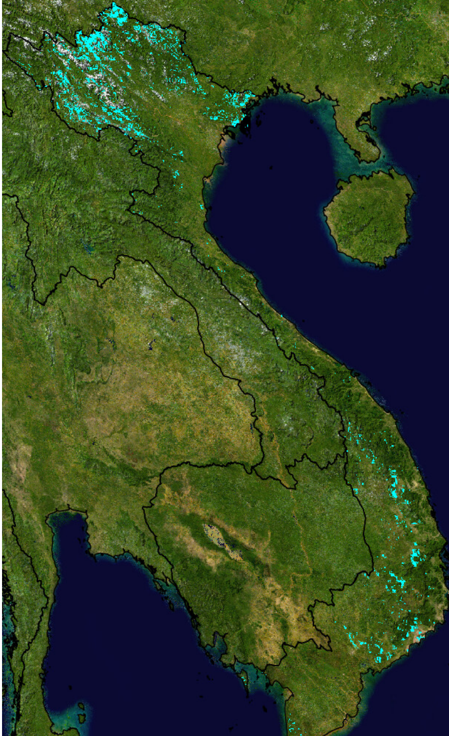
Figure 8: Restoration of 20% of deforested lands. Priority locations for restoration (cyan) for a solution that represents a balance between climate change mitigation and biodiversity conservation objectives while maximising cost-effectiveness (benefit/cost).
