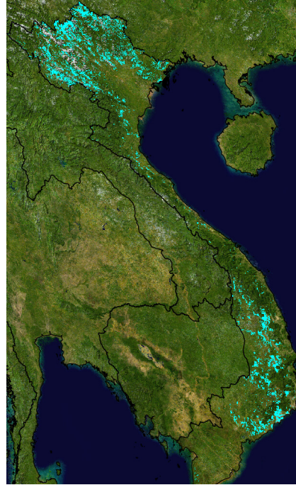
(b) cost-effective: biodiversity conservation
