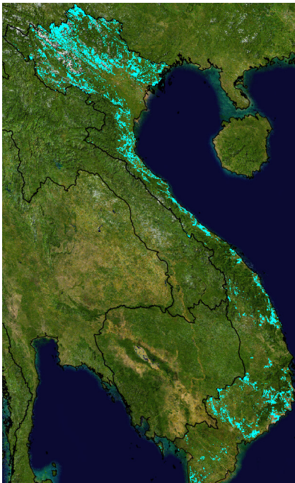
(c) max-benefit: climate change mitigation
