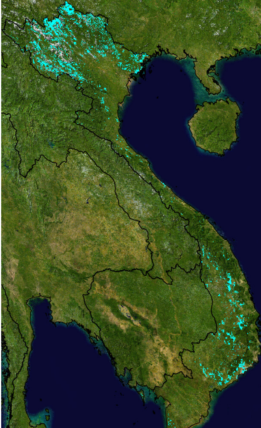
Figure 11: Restoration of 30% of deforested lands. Priority locations for restoration (cyan) for a solution that represents a balance between climate change mitigation and biodiversity conservation objectives while maximising cost-effectiveness (benefit/cost).
