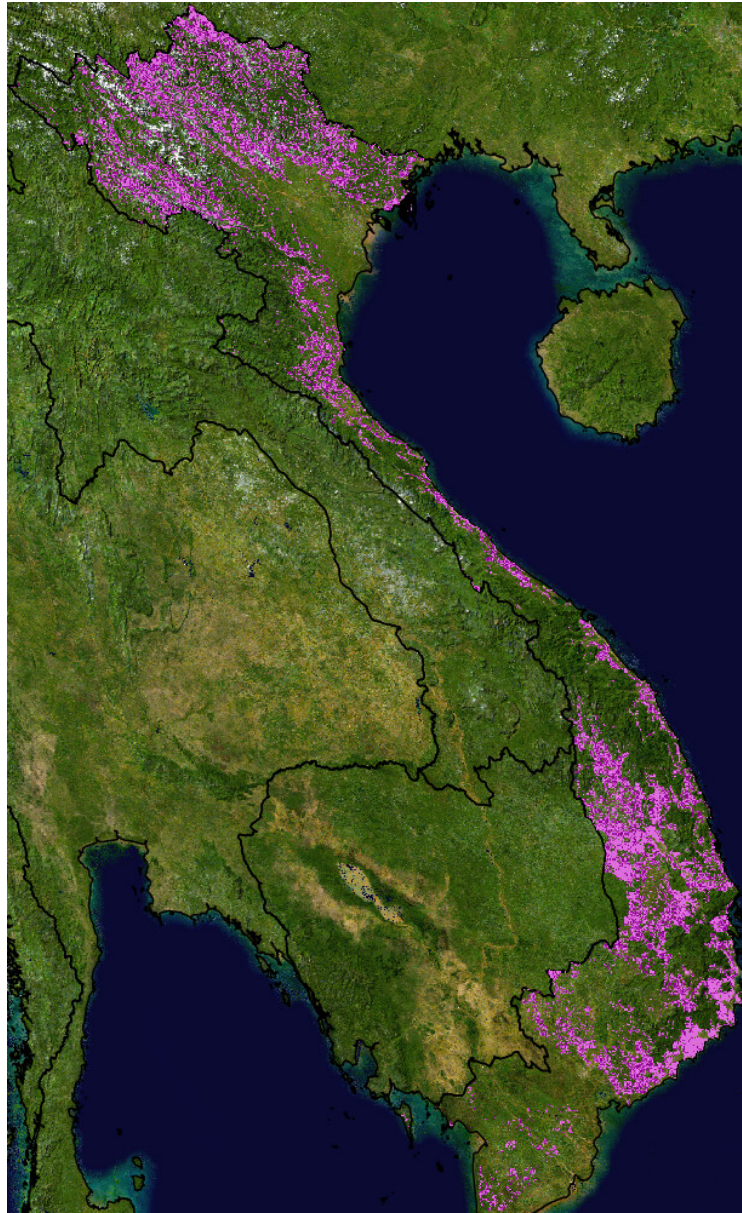
Figure 2: Area deemed available for forest restoration. Areas in purple indicate the 1 km 2 planning units that were assessed to have potential for forest restoration given (see Methods for details). The shading of cells from light to dark purple is proportional to the area within each planning unit available for forest restoration.
