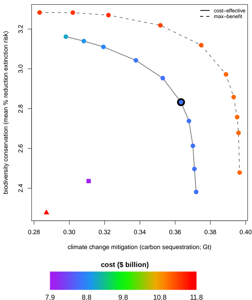
Figure 13: Restoration of 40% of deforested lands. Performance of a range of forest restoration prioritisation scenarios (points) with respect to climate change mitigation benefit (x axis), measured as above-ground carbon sequestration, and biodiversity conservation benefit (y axis), measured as the mean percent reduction in extinction risk among all species. Cost-effective scenarios (solid line) maximise return-on-investment (benefit/cost) and are likely to represent the most feasible restoration planning options. For reference, maximum-benefit scenarios (dashed line) that maximise returns irrespective of cost are also presented. The point circled in black represents a potential good compromise solution. Two further reference scenarios are also presented in which restoration is allocated randomly (triangle) or to minimise costs irrespective of benefit (square). For all scenarios the colour represents the total cost of the solution (USD; see legend). Maps of the locations associated with several of these solutions are included in the following two figures.
